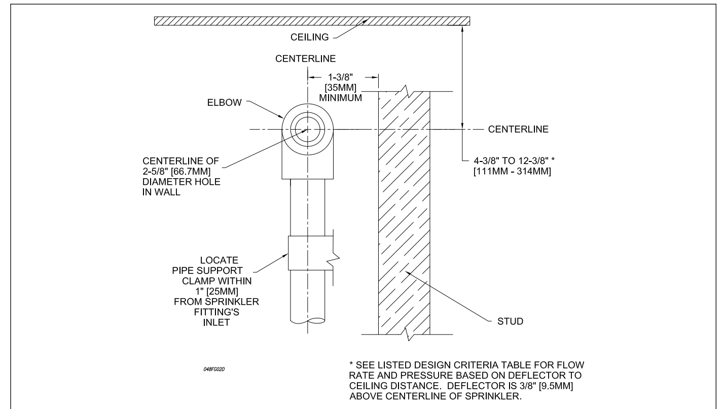
Fig. 2 Front View
