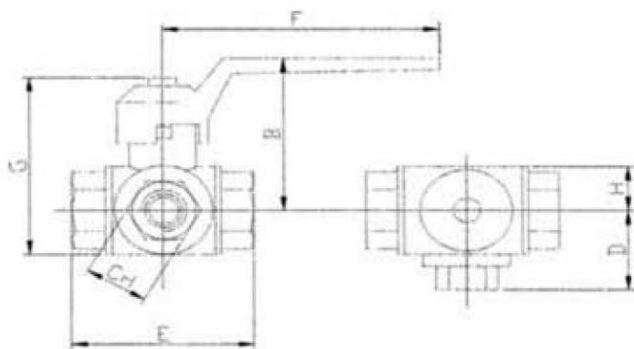
T-Port Configuration
