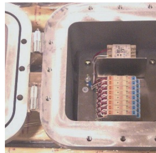
GAUGE POWER SUPPLY WITH ZENER BARRIERS
