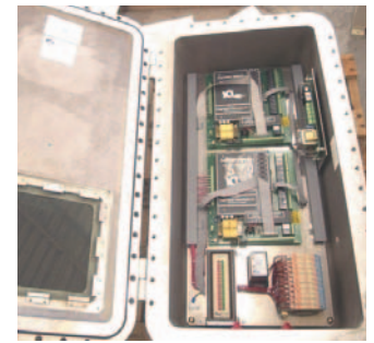
LEVEL ELECTRONICS WITH ZENER BARRIERS
